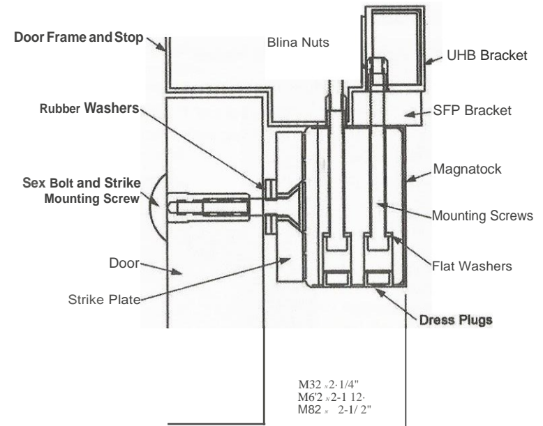
Figure 2. Magnalock Installation on an Out-Swinging Door
