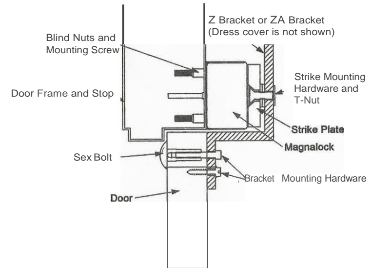
Figure 3. Magnalock Installation on an In-Swinging Door
