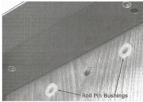
Figure 13. Installing the Roll Pin Bushings
