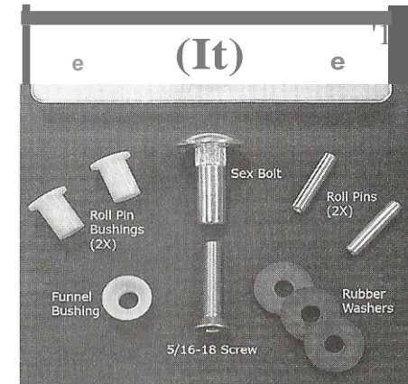
Figure 11. Strike Plate Components
